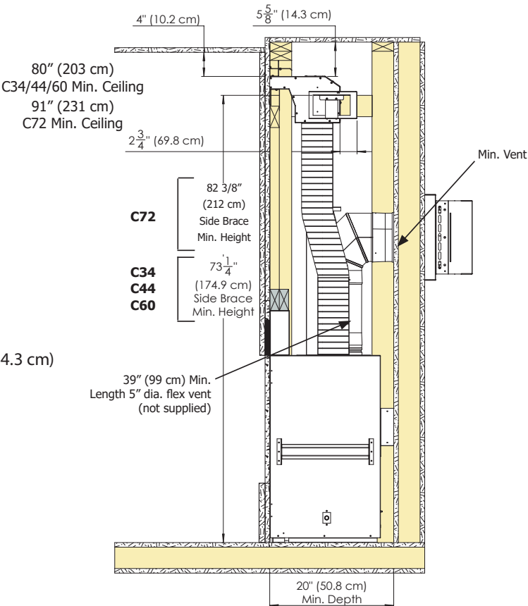
Figure 8: C44 CSS Front Vent Kit - Min. Install
