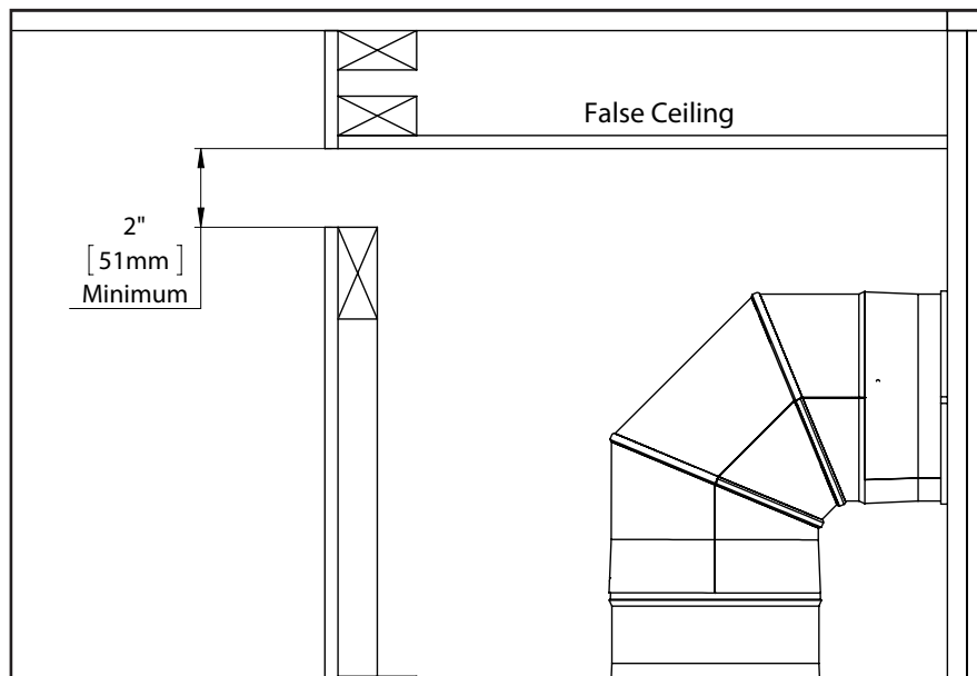
Figure 3: False Ceiling
