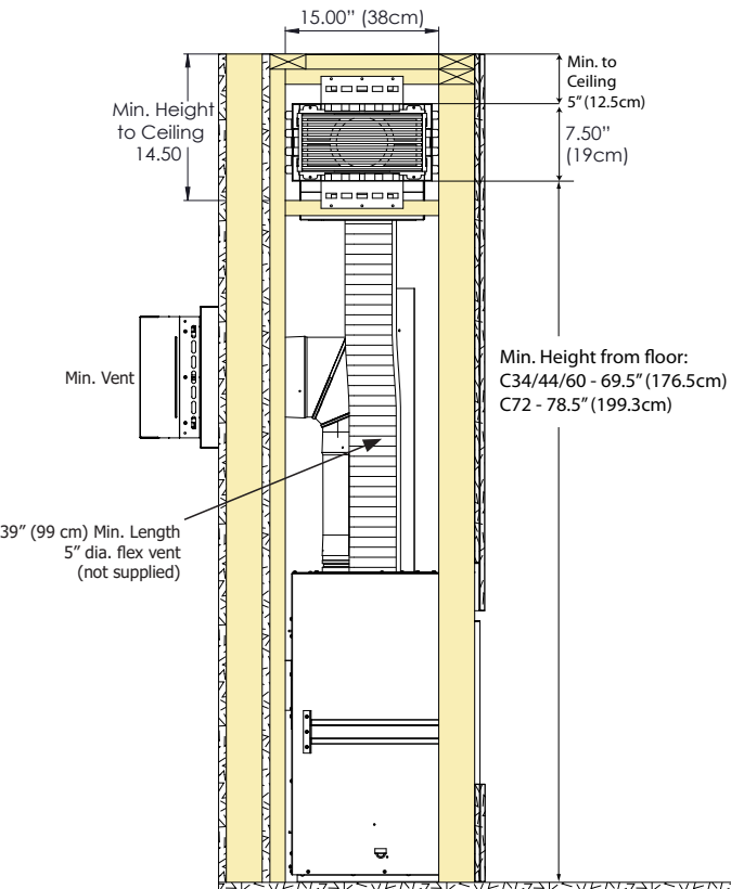
Figure 9: C44 CSS Side Vent Kit - Min. Install
