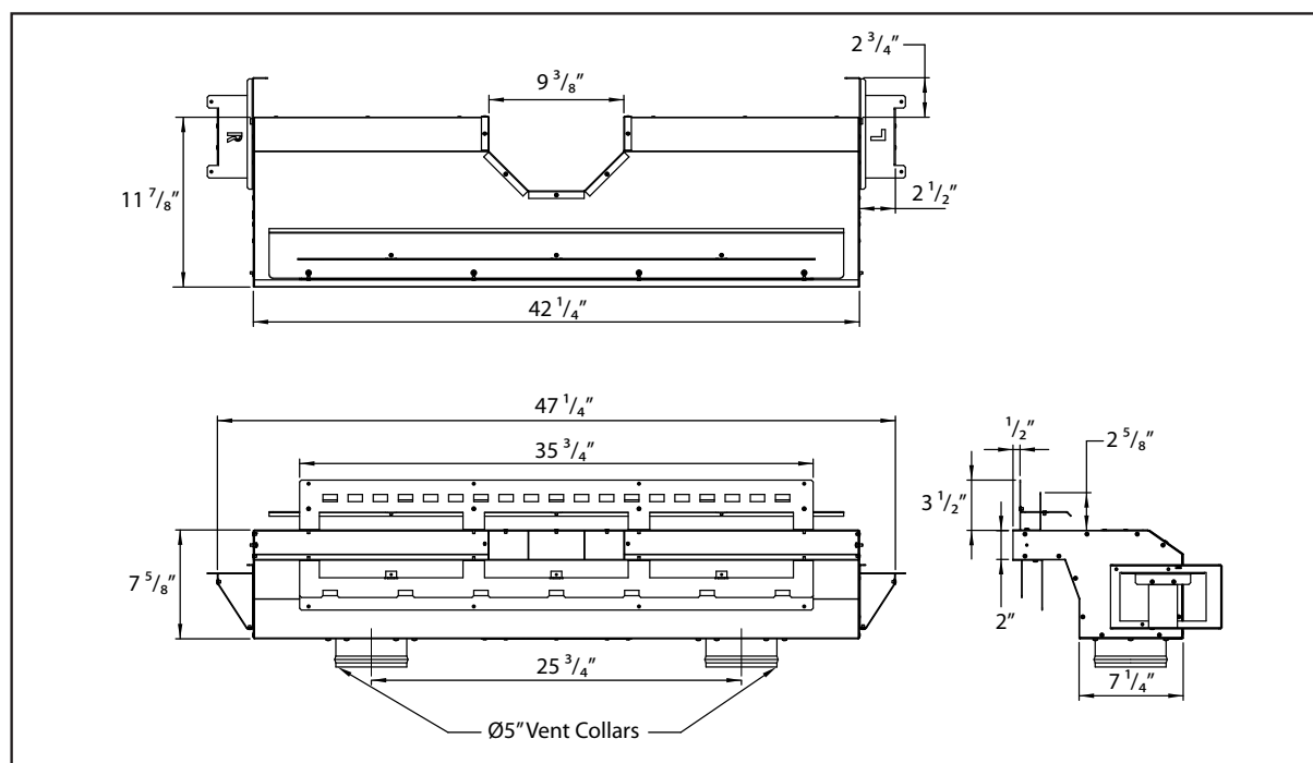
Figure 7: C44 CSS Front Vent Kit - Dimensions
